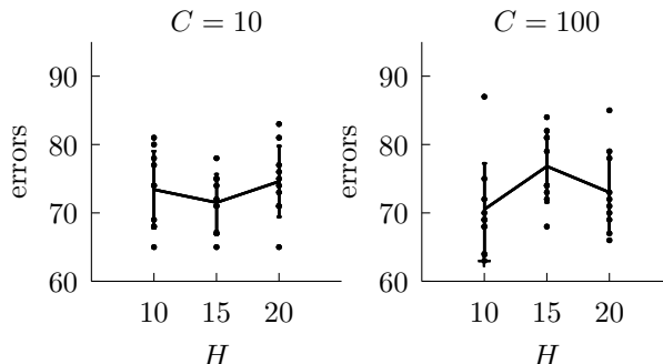
Figure 3: Results for the networks on the Pima Indians data-sets for C = 10 and C = 100 ( C = 1 is not shown due to space constraints). Dots represent each of the ten different networks initialisations. The network which achieved the overall minimum error is marked with + . Also shown is the mean and error-bars at one standard deviation for each parameterisation.
