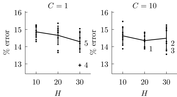
Figure 5: Results for the networks on the FISH data-sets for C = 1 and C = 10 . Dots represent each of the ten different networks initialisations. The networks with the five lowest validation set error are marked in order 1 to 5, with 1 having the lowest validation error.
