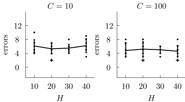
Figure 4: Results for the networks on the Leptograpsus crabs data-sets for C = 10 and C = 100 (once again C = 1 is not shown but is similar).
