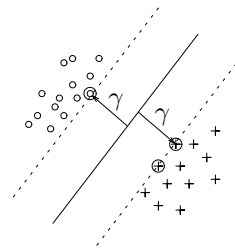
Figure 2: In linearly separable data, maximum margin provides a unique solution. Circled data-points indicate the support vectors and \gamma indicates the size of the margin.
